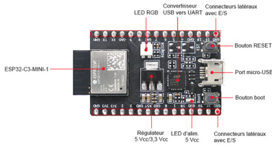
ESP32-C3-DevKitM-1
